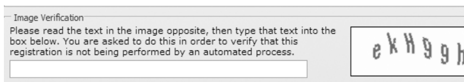
Figure 1 Text-based CAPTCHA
